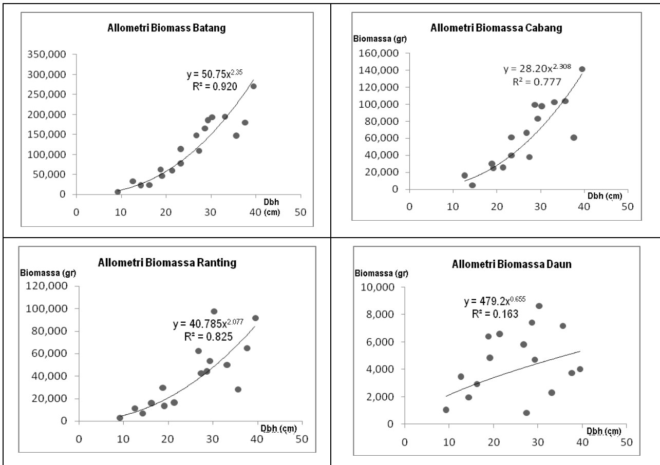
Gambar 3. Grafik allometri bagian pohon (batang, cabang, ranting, daun) dengan dbh Figure 3. Graphic of allometry between trees component with dbh
