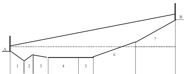
Gambar 1. Sketsa jalur kabel Figure 1. Sketch of cable way
