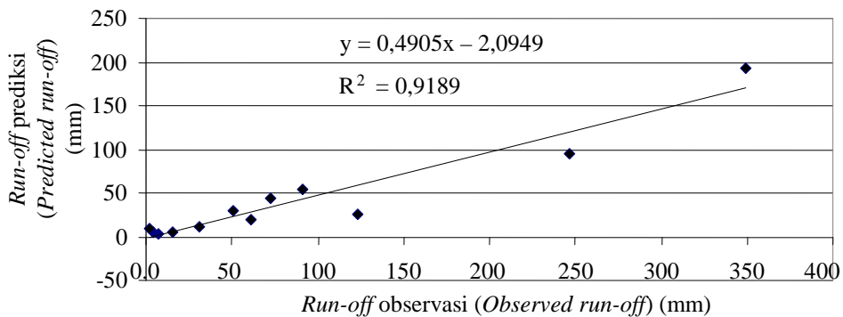
Gambar (Figure) 10. Hubungan antara pengamatan dan prediksi aliran sub DAS Wuryantoro tahun 2007 (The relationship between observation and prediction of run-off in the Wuryantoro sub watershed in 2007)
